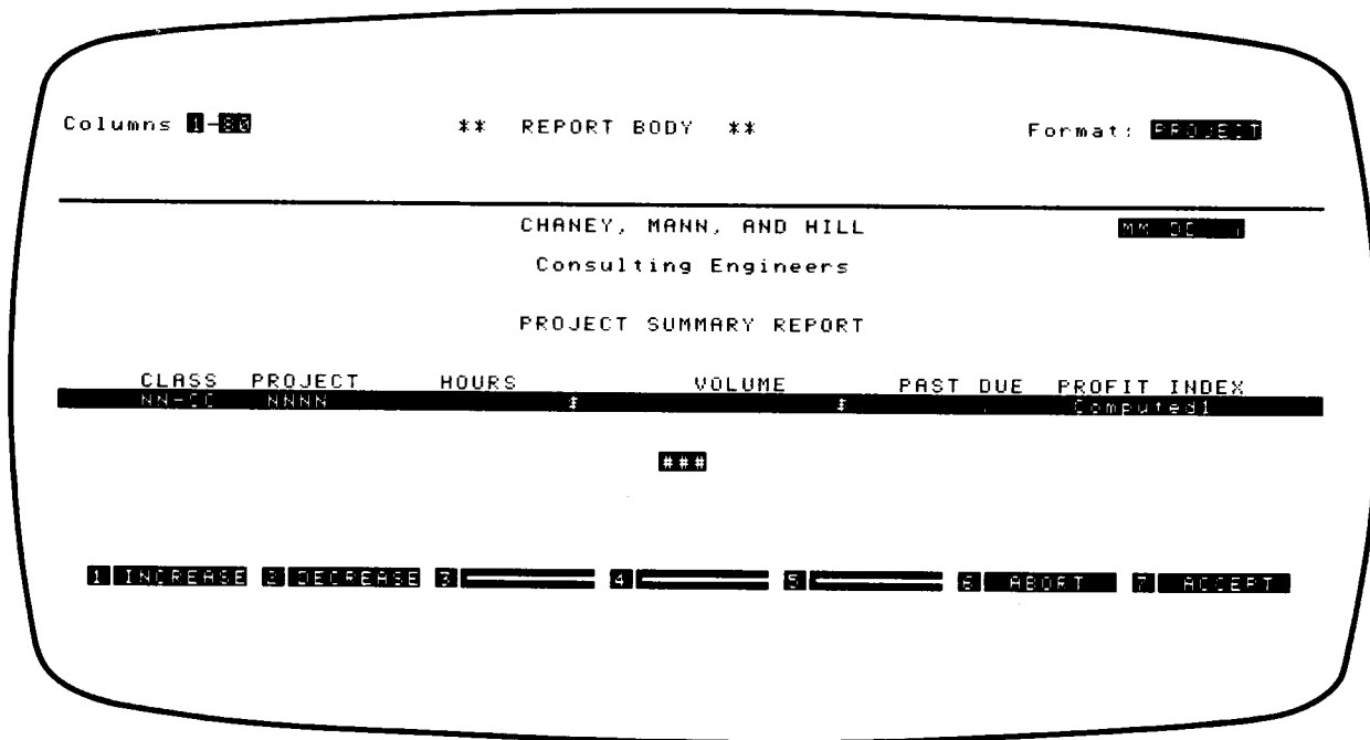
FILE/80 Display
