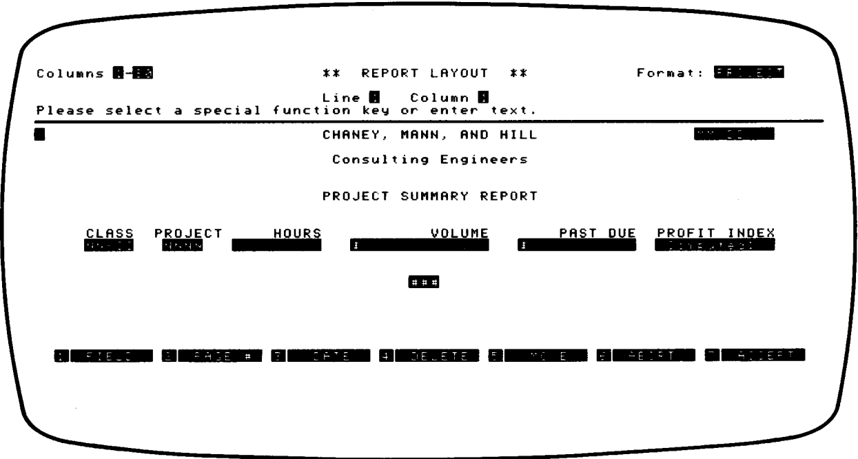
FILE/80 Display
