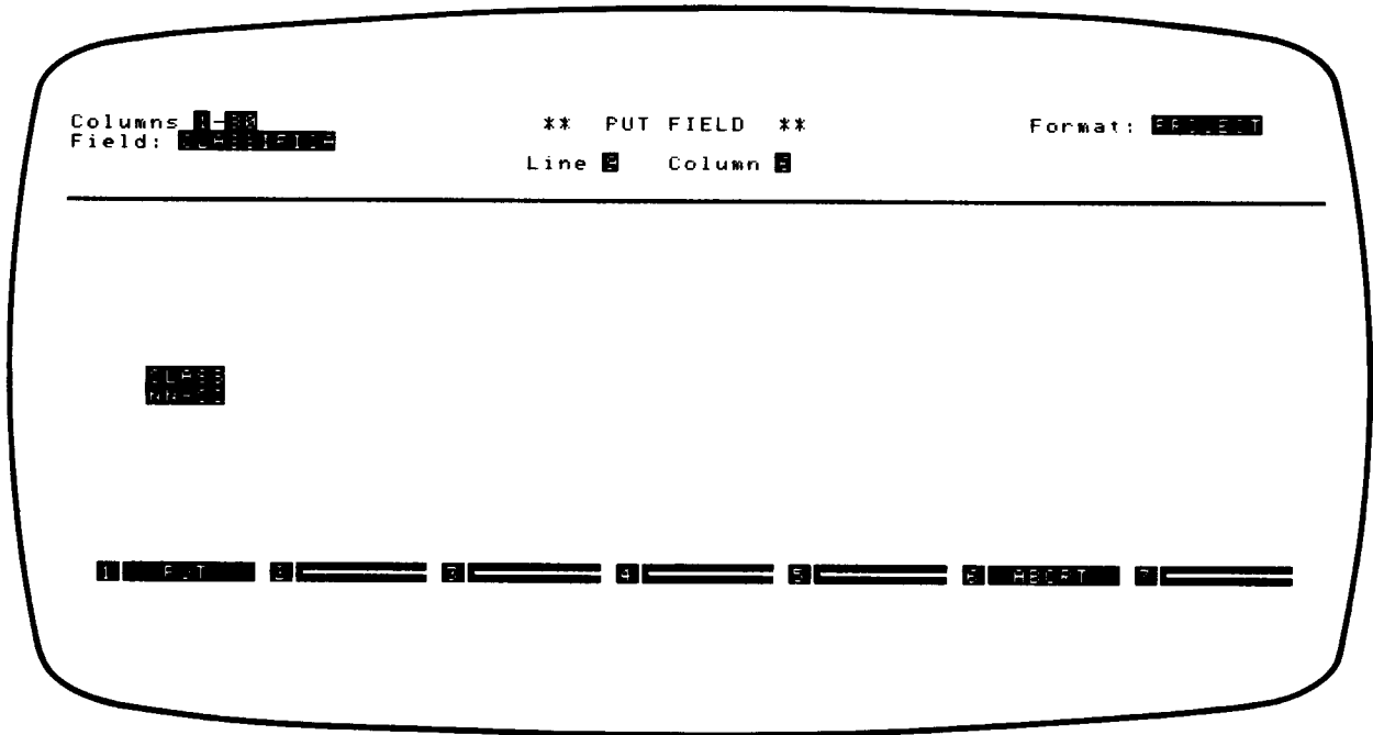
FILE/80 Display
