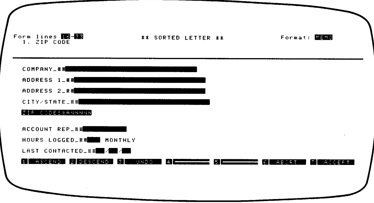
FILE/80 Display
