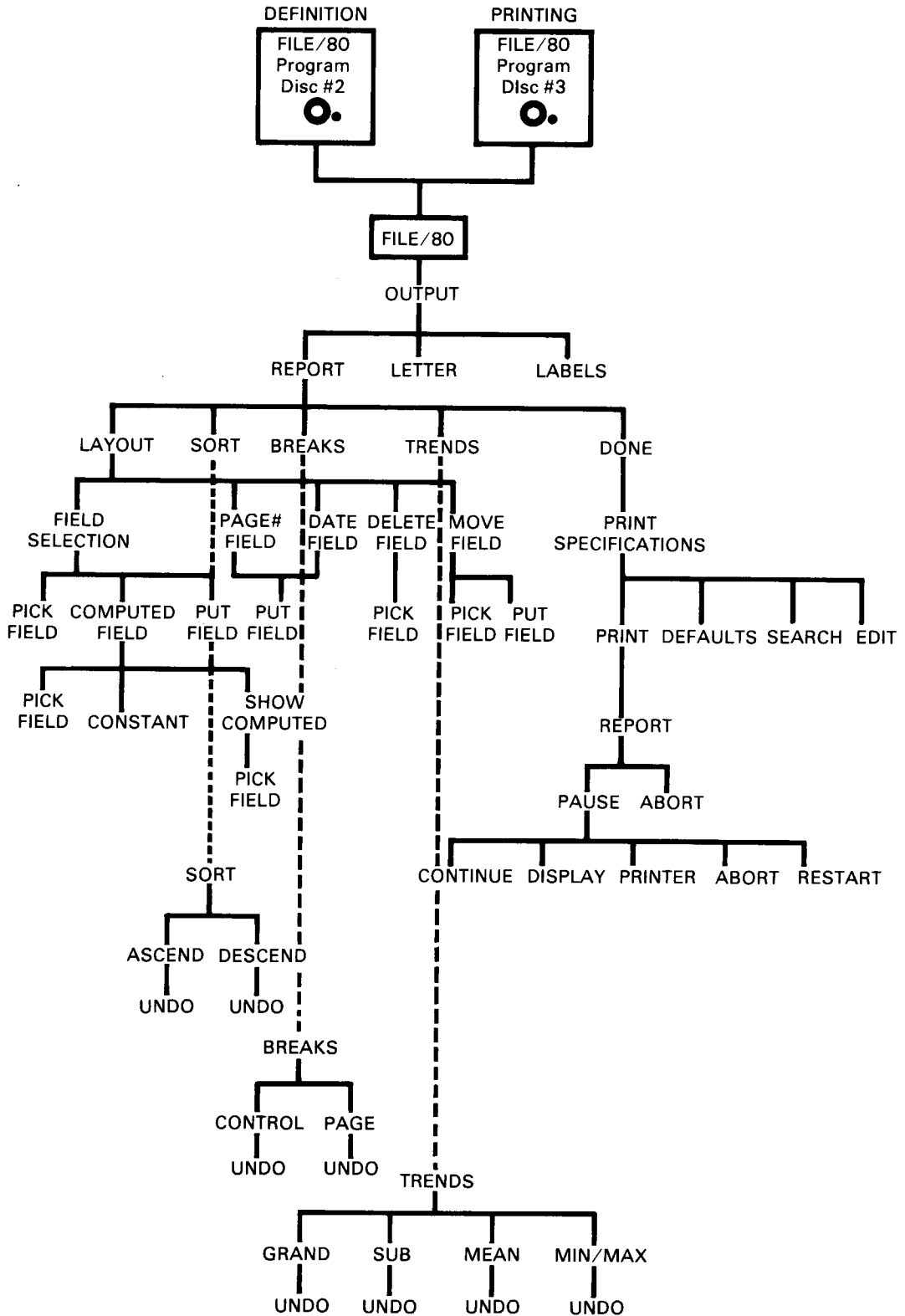
REPORT Diagram
