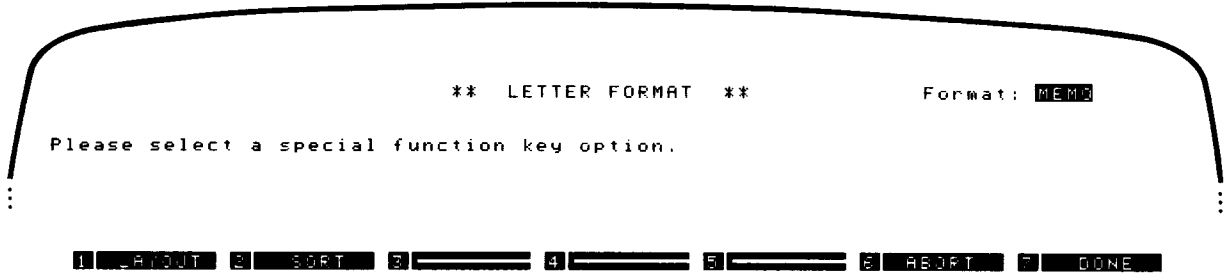
FILE/80 Display
