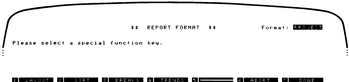
FILE/80 Display
