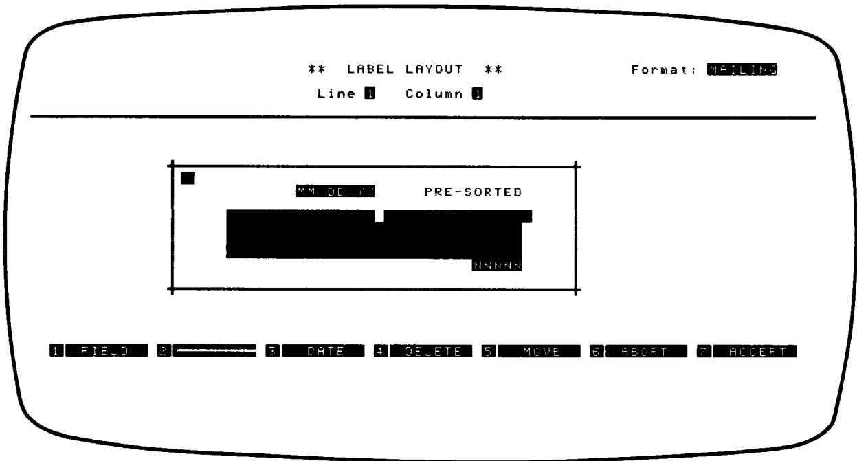
FILE/80 Display
