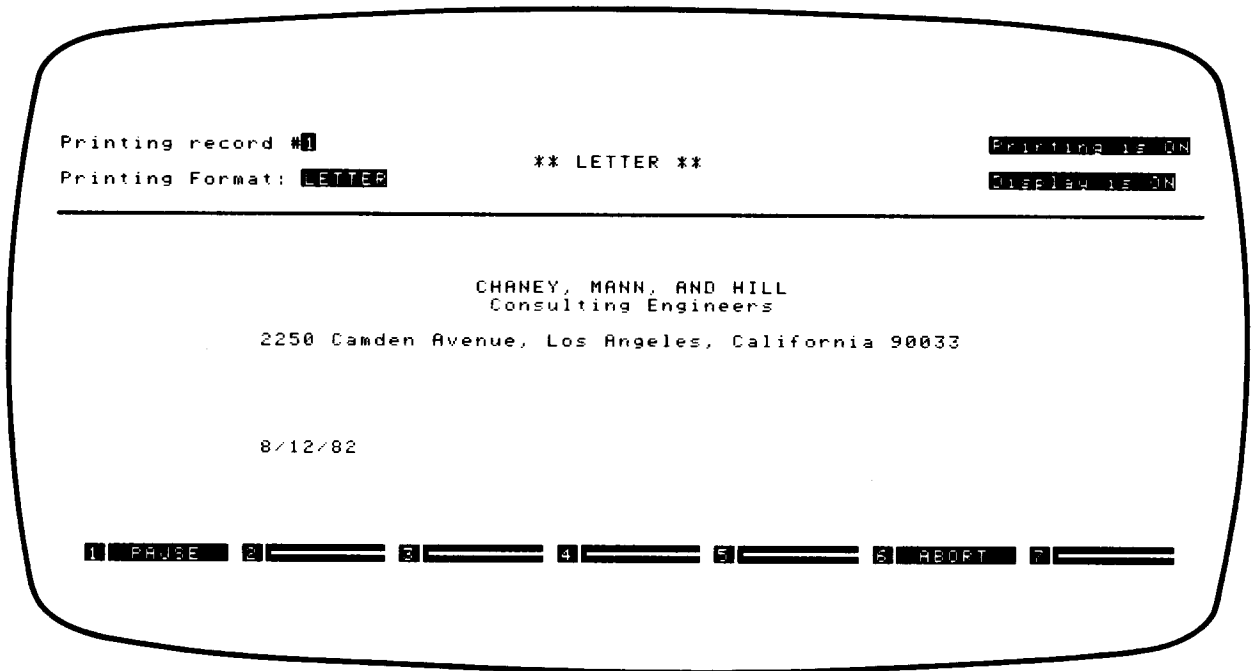
FILE/80 Display
