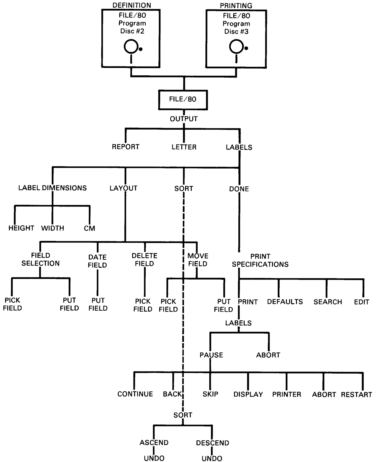
LABELS Diagram
