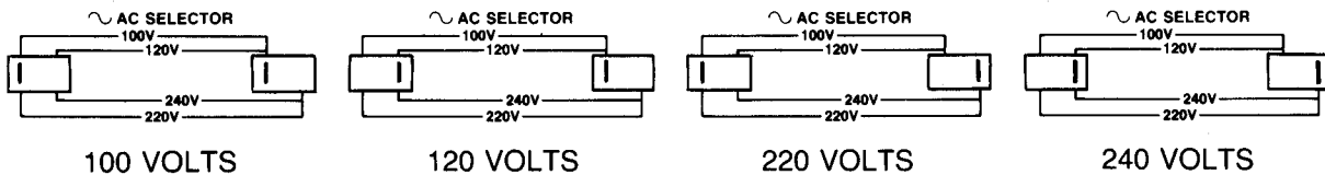
Figure 2-1. Line Voltage Select Switches
