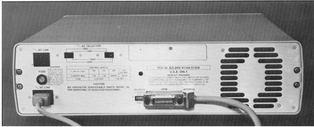
Figure 2-5. Interface Connection
